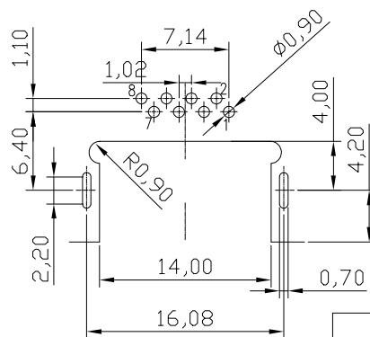
PCBLAYOUT TOP VIEW TOL:±0.05
