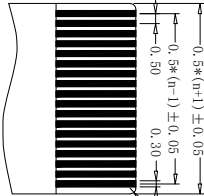
PROPER CABLE (SCALE 2:1)
