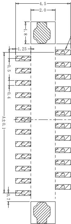
PCB LAYOUT TOLERANCE: ±0.05
