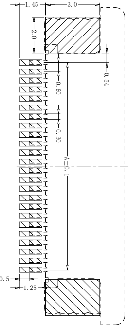
PC BOARD LAYOUT
