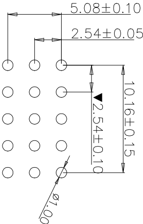
Recommended P.C.B Layout(±0.05)
